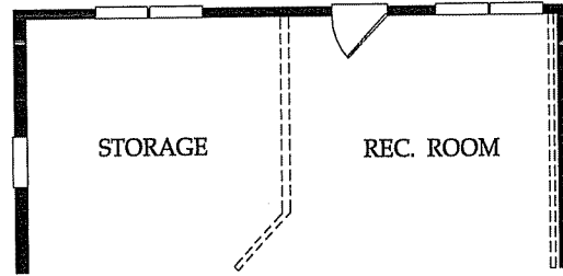
Partial Basement with Optional Sunroom at Walkout Condition
