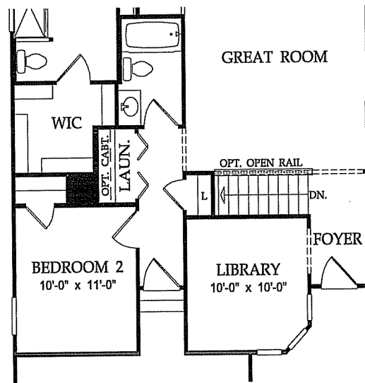
Partial First Floor with Optional Basement
