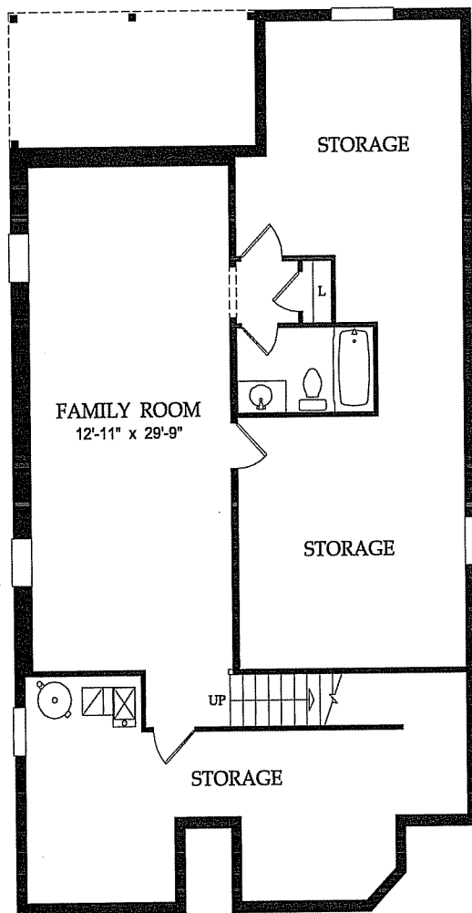
Optional Walkout Basement
