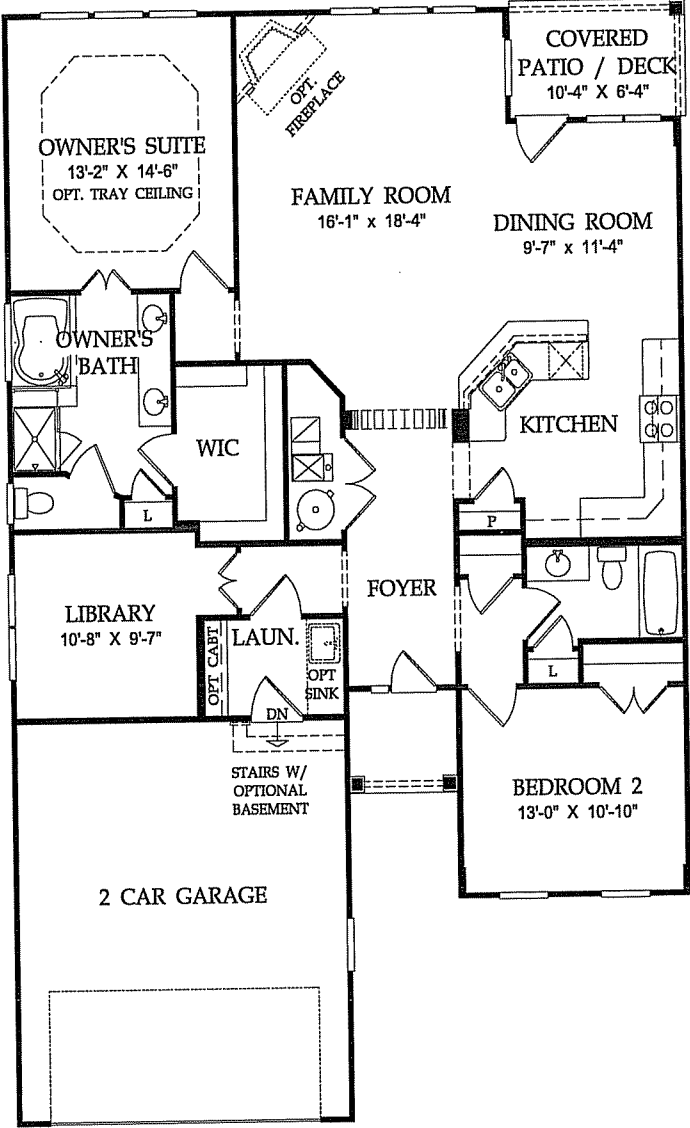
Partial First Floor with Optional Basement
