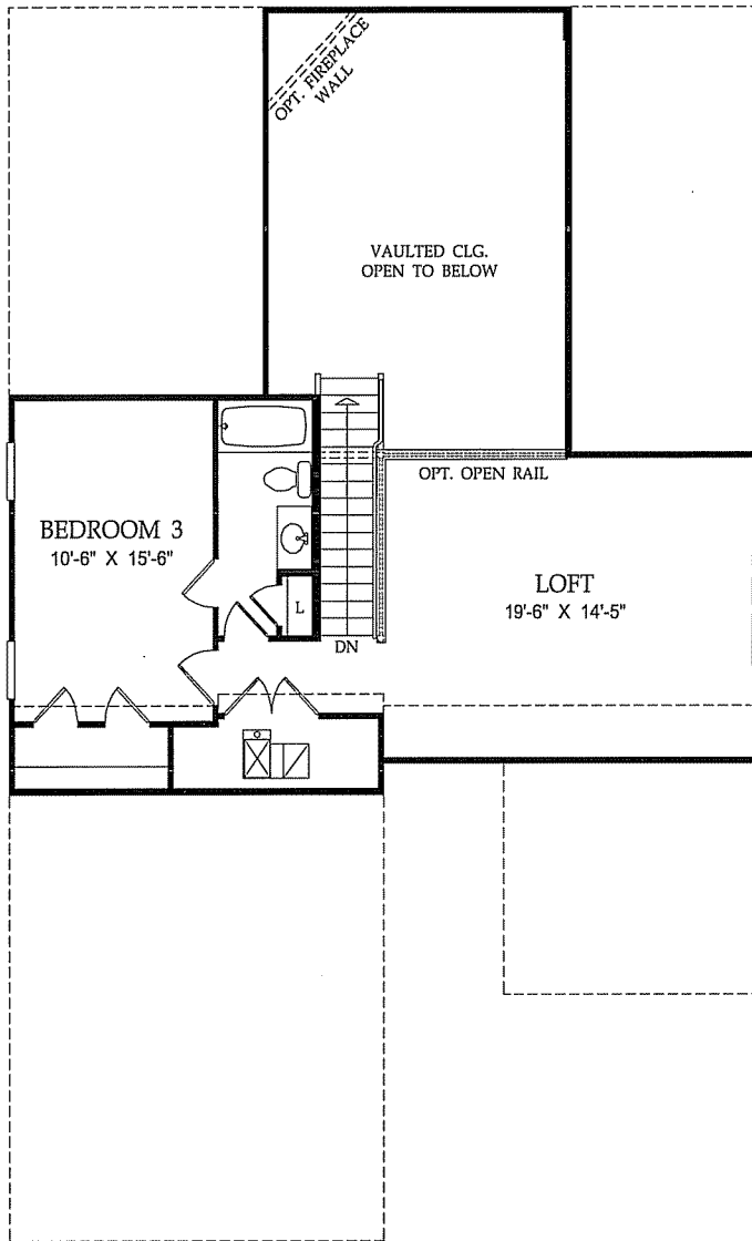
Second Floor
