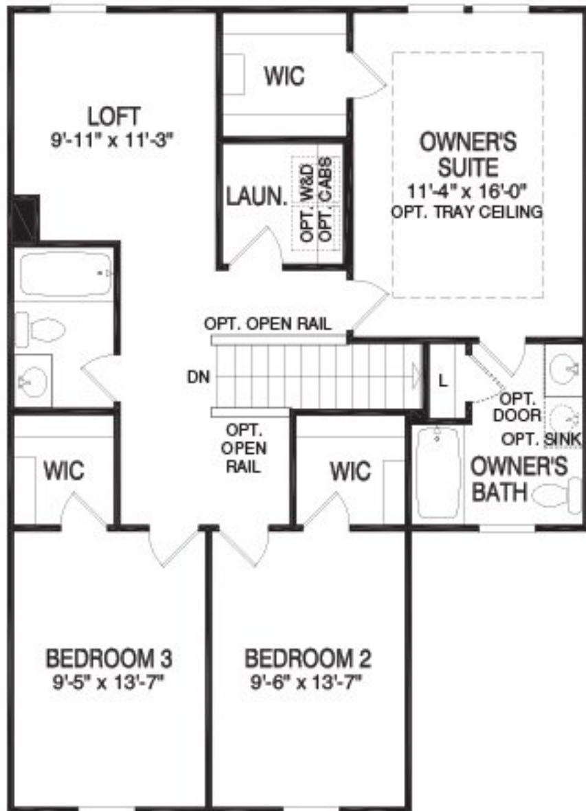
Second Floor w/ Opt. Basement Condition
