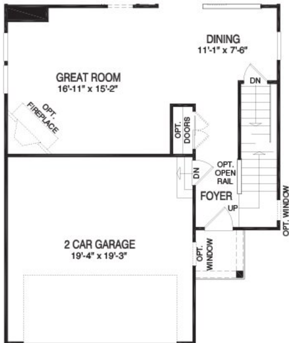
First Floor w/ Optional Basement
