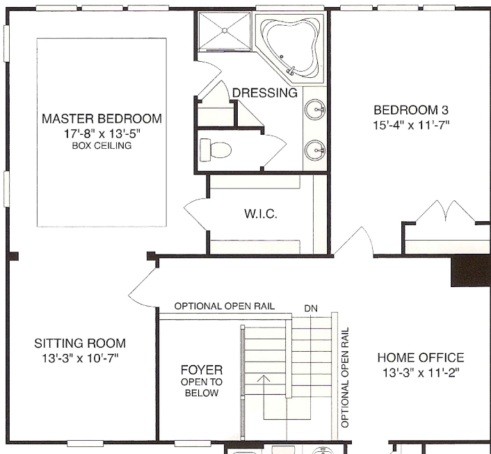
ALTERNATE SECOND FLOOR PLAN
