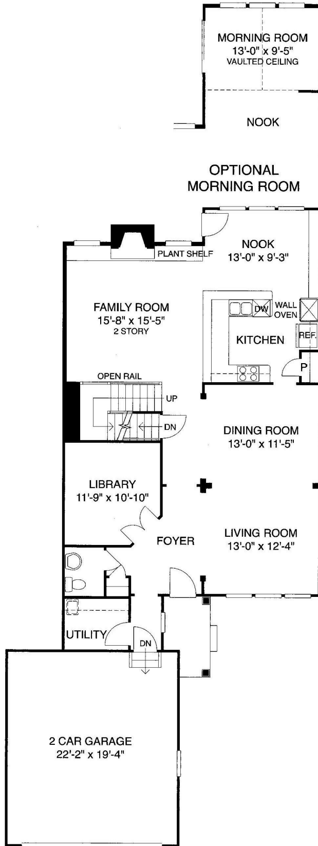
FIRST FLOOR WITH ELEVATIONS 1-4
